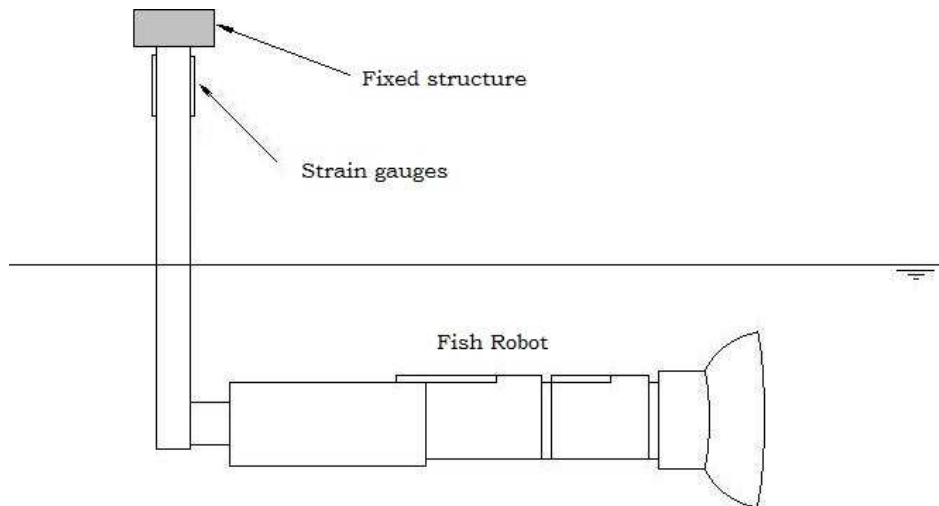
Figure 2. Test facility to study propulsion forces of Tucuzul I
